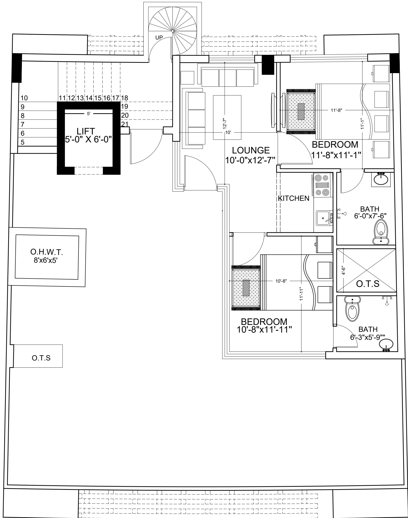
TOP ROOF FLOOR PLAN MUMTY AREA 803 sq ft
